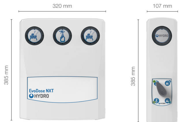
EvoDose NXT 1 Button and QDV: 107mm x 120mm x 385mm
