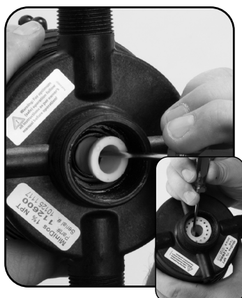
Step 7. Replace #82 SHAFT SEAL SPACER and #16 Gasket.
