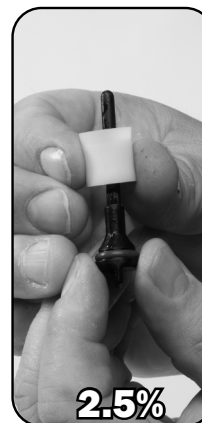
Step 3. Replace #44 DOSAGE PISTON thin lips up. Clean & inspect #14 O-ring replace if necessary.
