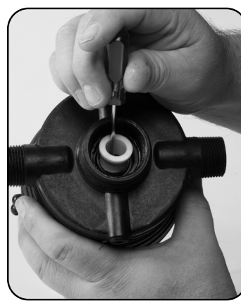
Step 3. Remove #83 SHAFT SEAL SPACER.
