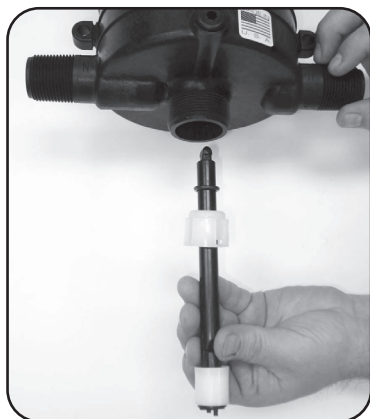
Step 6. Reinsert #15 SEAL RETAINER and #17 O-ring onto #51 SHAFT ASSEMBLY.
