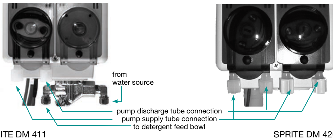
Figure 2-3 Flush Manifold Connection
